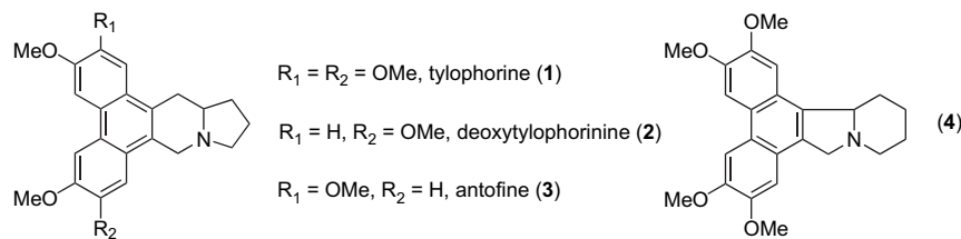
Figure 1. Structures of alkaloids (1), (2), (3), and their analogue (4).
