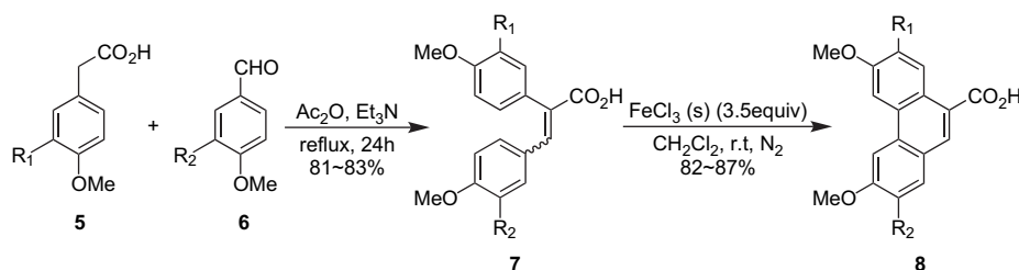
Scheme 1. Synthesis of the compounds 7 and 8 .
