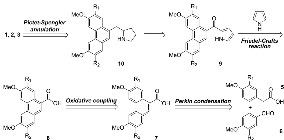
Scheme 2. Retrosynthetic analysis of phenanthroindolizidine alkaloids 1 , 2 , and 3 .
